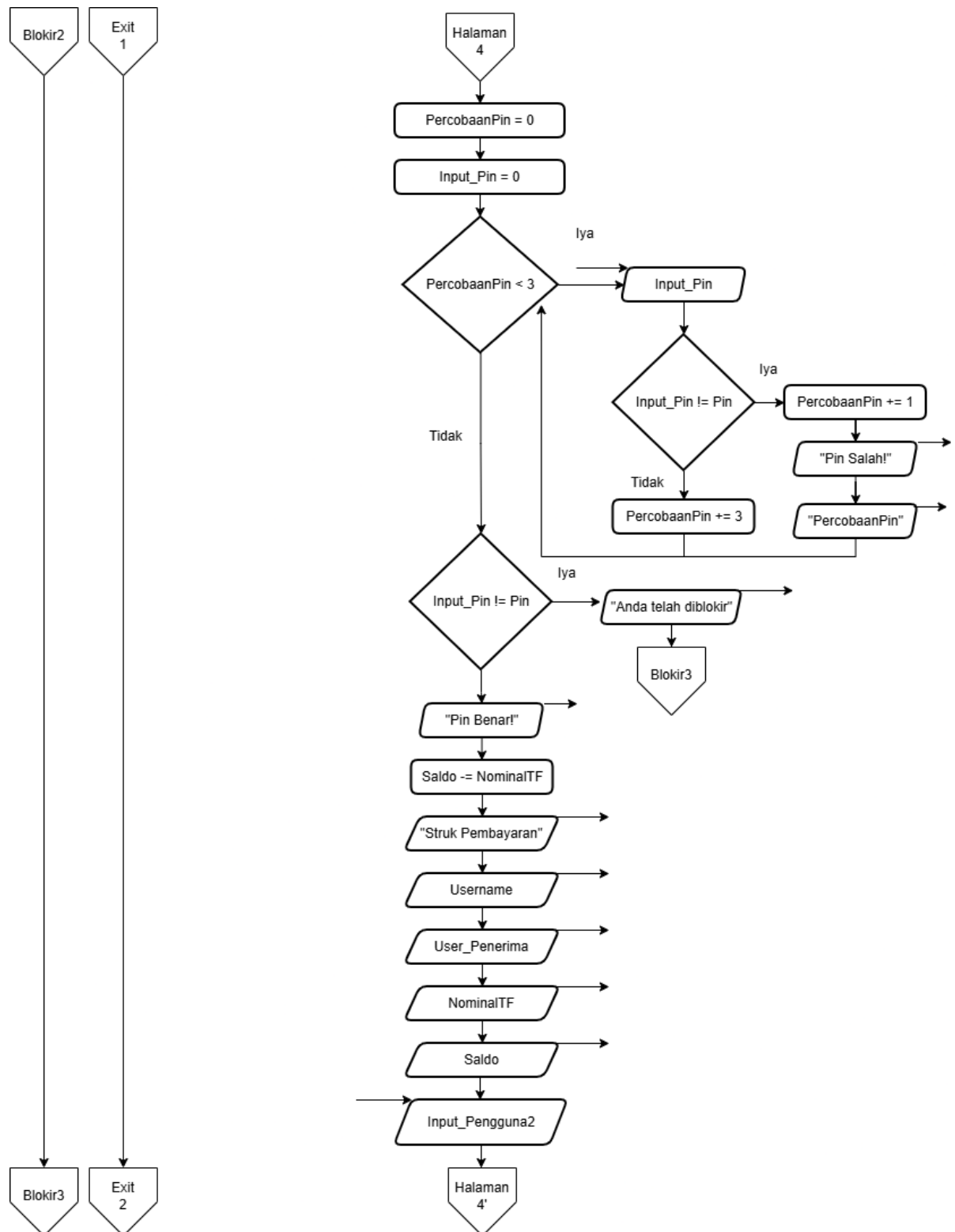
Gambar 1.4 Halaman 4 Flowchart
